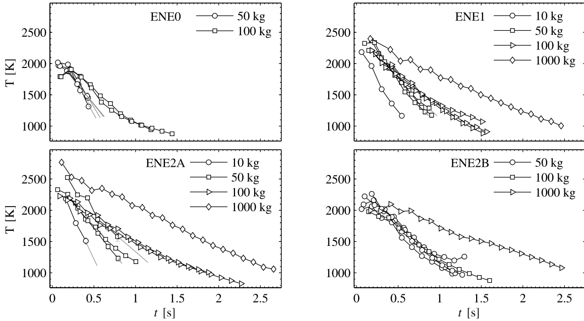
Figure 44: Temperature versus time curves obtained by fits to fireball spectra of 10 (○), 50 (□), 100 (▷), and 1000 kg (◇) charges of various ENEs. Not all HE sizes were represented in each class of explosive. Grey lines represent linear extrapolations to T = 1200 K for those events in which the final temperature was greater than T = 1200 K.
