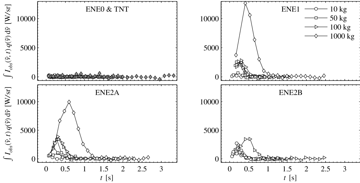
Figure 54: Time-resolved intensities at unknown emission frequencies for each HE type detonated during the Brilliant Flash II field test. The intensity was integrated over q(\tilde{\nu}) where q = 1 if 6535 \leq \tilde{\nu} \leq 6554 \text{ cm}^{-1} or 6587 \leq \tilde{\nu} \leq 6598 \text{ cm}^{-1} and q = 0 otherwise. Both the ENE0 (white) and TNT (grey) intensities are provided in the top left panel.
