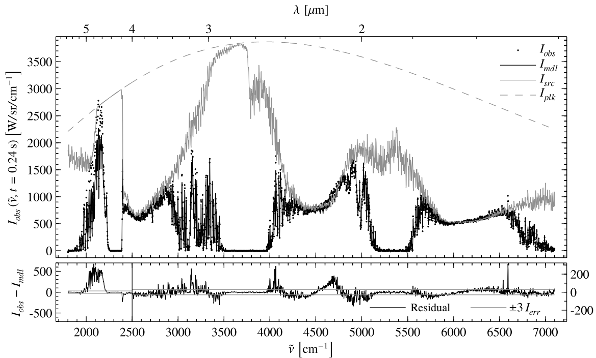
Figure 27: Top panel: Observed fireball spectrum ( \cdot ) at t = 0.24 s from a 50 kg ENE2B detonation compared with the best fit of the fireball model to \tilde{\nu} > 2500 \text{ cm}^{-1} (solid black). The estimated at-source spectrum is provided (solid grey) along with the Planckian intensity distribution (dashed grey). Bottom panel: Fit residuals ( I_{obs} - I_{mdl} , black) compared with I_{err} (grey), which is an estimate of the instrument noise level. The left ordinate is used for \tilde{\nu} < 2500 \text{ cm}^{-1} and the right ordinate corresponds to \tilde{\nu} \geq 2500 \text{ cm}^{-1} .
