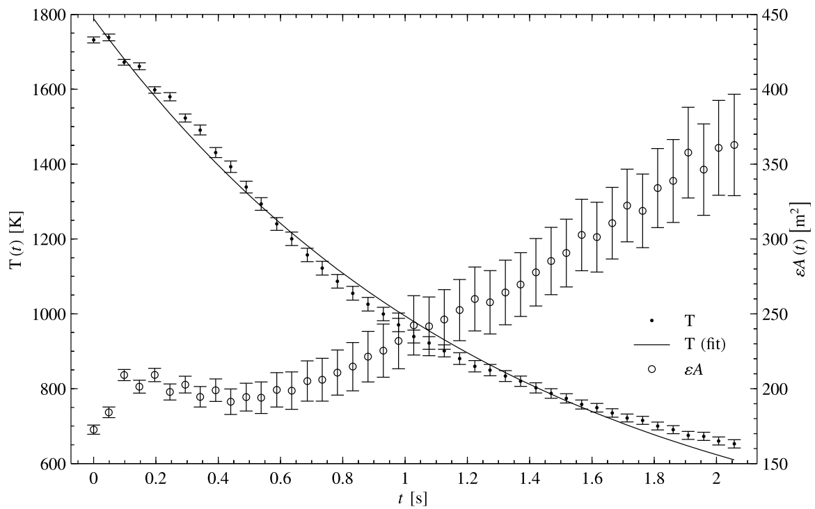
Figure 14: Spectral estimates of temperature ( \bullet ) and emissive area ( \circ ) plotted as functions of time for a small, type A CMM detonation fireball. The T -axis is on the left and the \varepsilon A -axis is on the right. Vertical error bars represent the statistical uncertainty (95% confidence interval) in the fit parameter. The solid black curve represents an exponential fit to the temperature curve.
