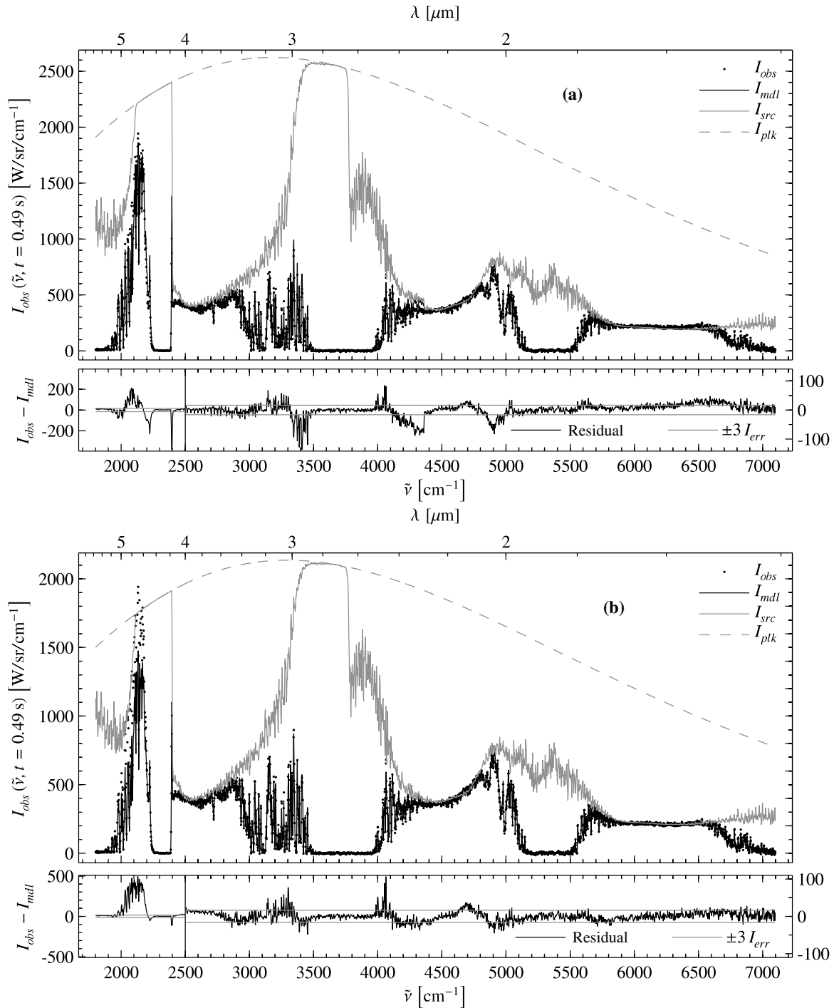
Figure 21: (a) Top panel : Observed fireball spectrum ( \cdot ) at t = 0.49 \text{ s} from a 50 kg TNT detonation compared with the best fit model (solid black). The estimated at-source spectrum is provided (solid grey) along with the Planckian intensity distribution (dashed grey). Bottom panel : Fit residuals ( I_{obs} - I_{mdl} , black) compared with I_{err} (grey), which is an estimate of the instrument noise level. The left ordinate is used for \tilde{\nu} < 2500 \text{ cm}^{-1} and the right ordinate corresponds to \tilde{\nu} \geq 2500 \text{ cm}^{-1} . (b) Same observed data, but fit and residuals obtained when fitting only to wavenumbers greater than 2500 \text{ cm}^{-1} .
