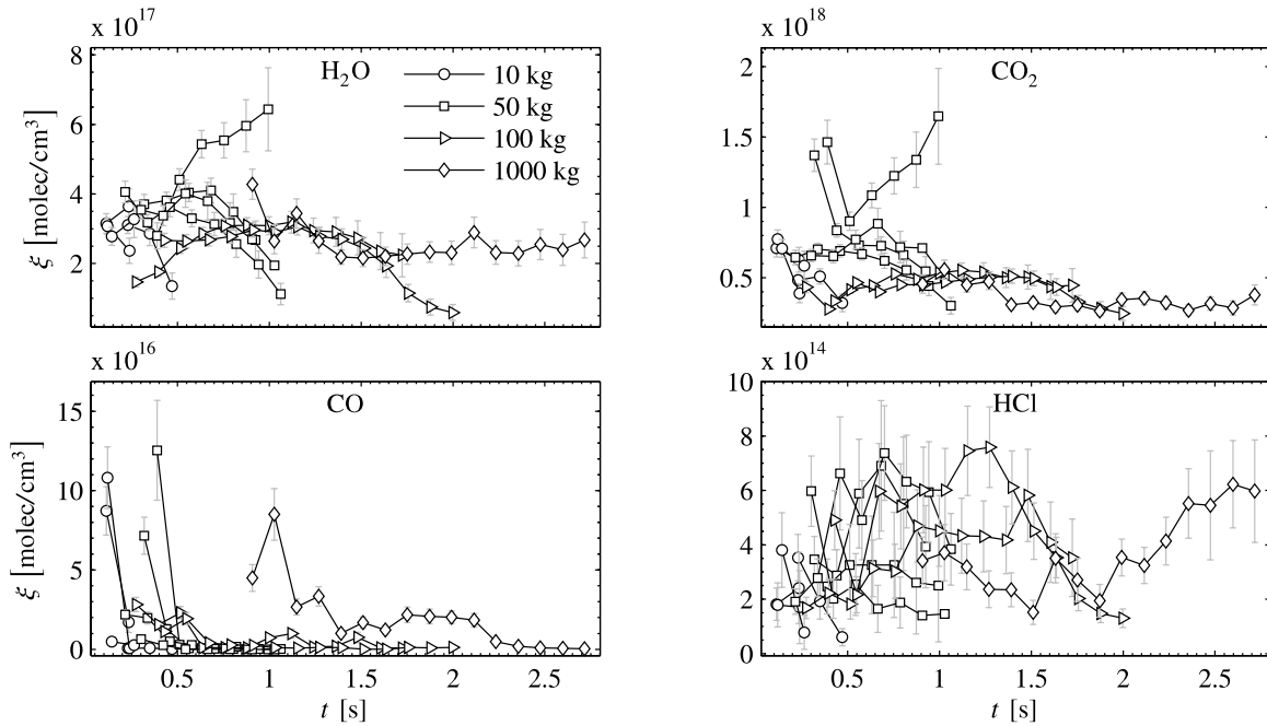
Figure 51: Concentration versus time profiles extracted from TNT fireballs for H 2 O, CO 2 , CO, and HCl. The different sized explosives are denoted in the following manner: 10 (○), 50 (□), 100 (▷), and 1000 kg (◊). The water and carbon dioxide values have been corrected for heated atmospheric contributions to the observed values. Concentrations extracted from spectra with the non-grey parameter satisfying G < 3 were omitted. Error bars represent fit parameter uncertainties (95% confidence level).
